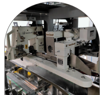
SEWING MACHINE
