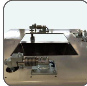
Net weigher
