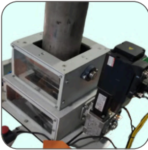
Gravity Feeder
