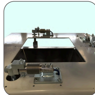
Net weigher
